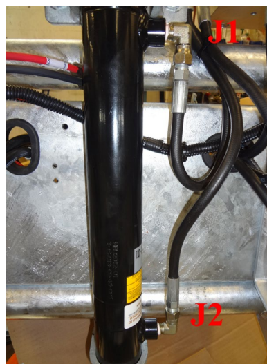
Jack hose installation (18" Hoses)
