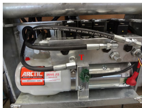
Wing plow power unit (P and T hoses installation 29")
